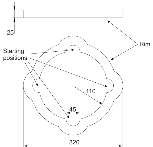
Figure 3 The removable rim viewed from the side and from above. Before commencing a trial, the subject should place the ball in a starting position (at front, back, left or right) by tilting the plate. All measurements are in millimetres.
