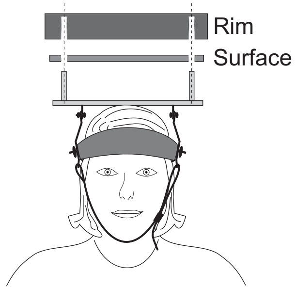
Figure 2 Exploded drawing of the neck coordination exercise device, including the removable rim and an exchangeable surface. Four different surfaces were used in order to vary the rolling resistance of the ball.
